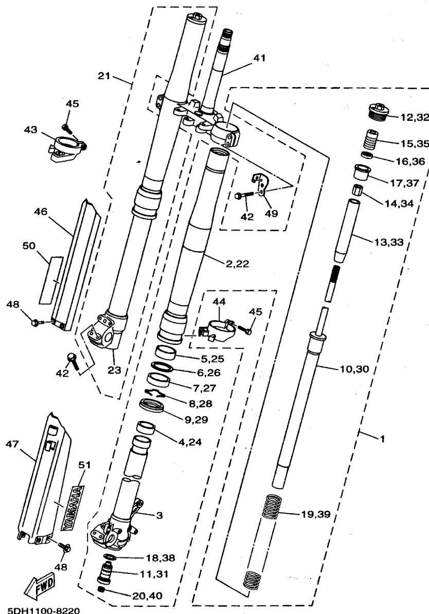
FIG. 22 FRONT FORK
