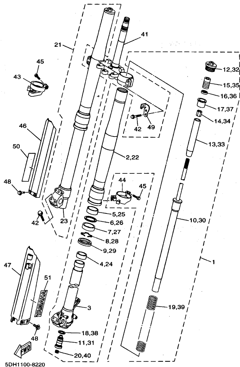
FIG. 22 FRONT FORK
